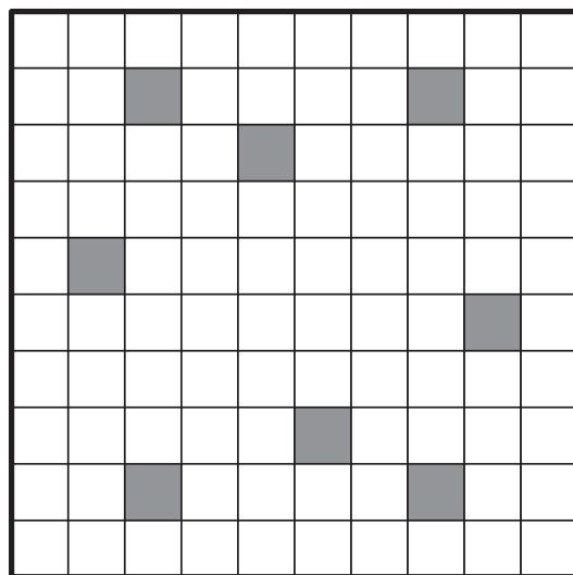
Common cells
