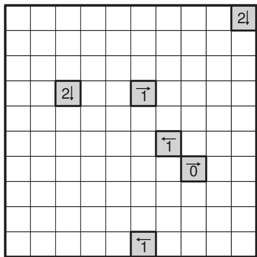
Yajilin
